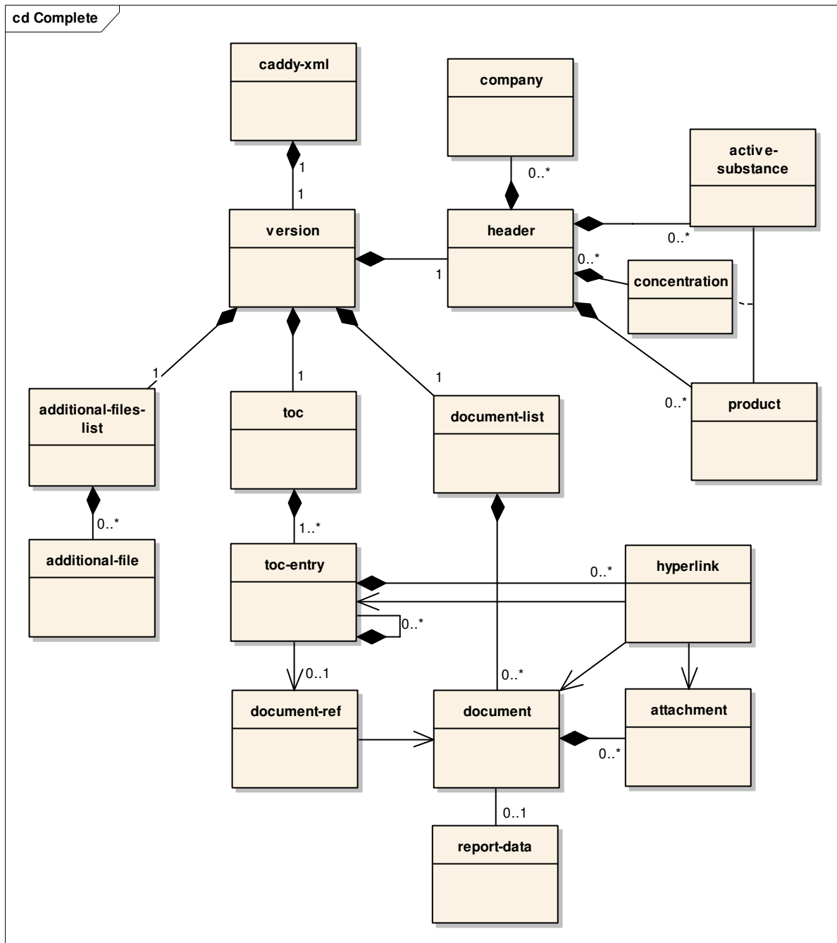
Figure 12: Overview CADDY-xml (v3) Elements
